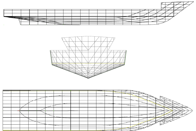
Figure 1: Lines Plan of the Parent Ship
