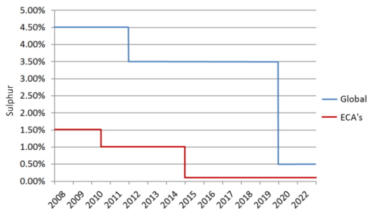
Figure 1: ECA regulations
